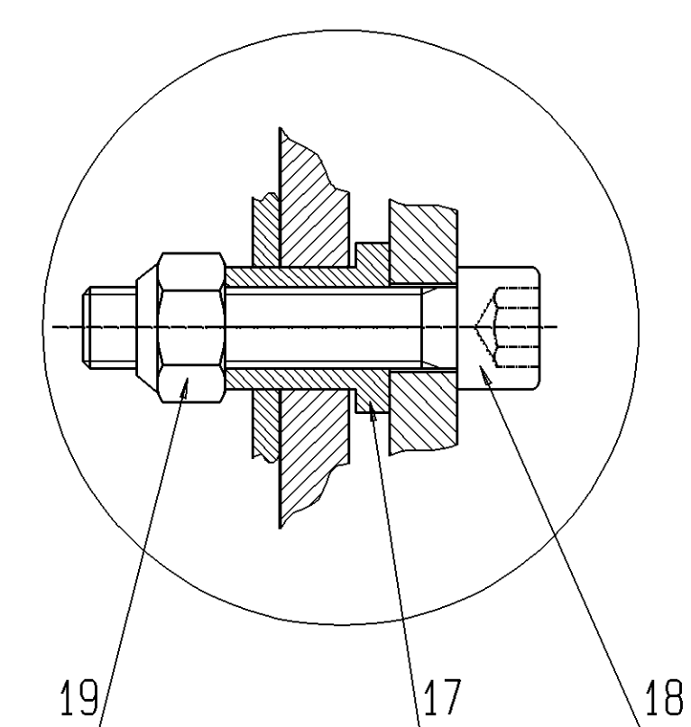
DETAIL I M/S=1:1
